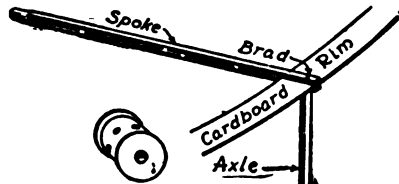
FIG. 156. — A Spool Hub for the Wheel.
